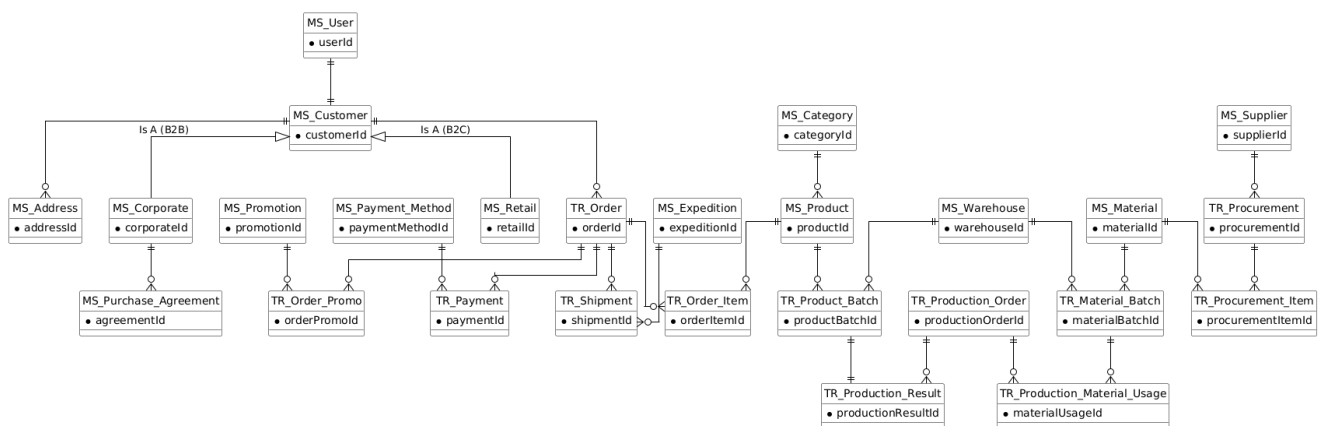
Gambar 3. Conceptual Entity Relationship Diagram (ERD)
